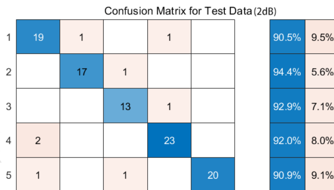
Figure 4: Confusion matrix for test data (2dB)
