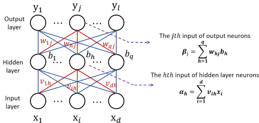
Figure 3: Forward propagation of the signal
