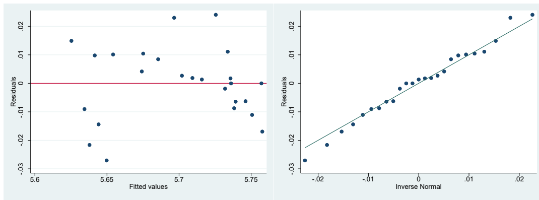
Figure 1: Residual vs fitted plot, and Normal Q-Q plot, STATA
