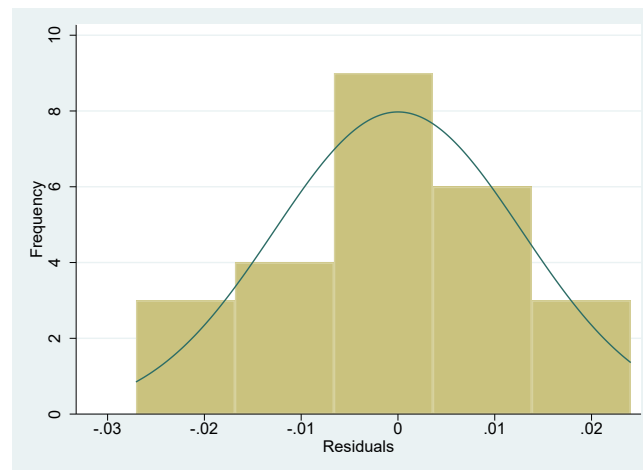
Figure 2: Histogram of residuals of multiple linear regression model, STATA
