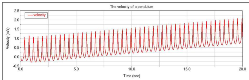
Figure 8: The relationship between pendulum's velocity and time when AUV descent.
