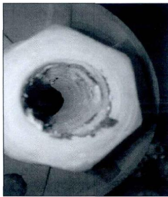
(a) Internal Thread Damage of GFRP Nuts (b) Surface Damage of GFRP Tendons
