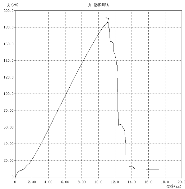
Figure. 3 Load-displacement Curve of Test Specimen S1
