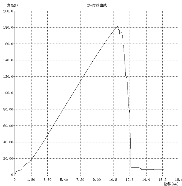
Figure. 4 Load-displacement Curve of Test Specimen S2
