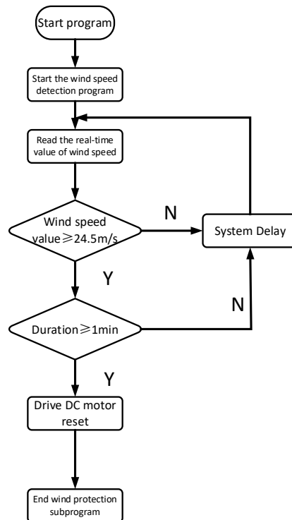
Figure 4: Flow chart of wind protection subprogram
