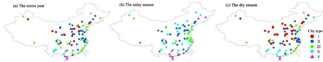
Figure 9: Temporal-spatial distribution characteristics of air-quality types at the different time scales.
