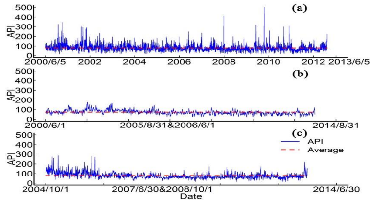
Figure 5: The typical characteristics of slight-pollution type. (a) Nanjing, (b) Chongqing, (c) Yangquan.
