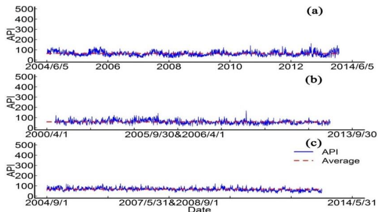
Figure 7: The typical characteristics of acceptable-quality type. (a) Liuzhou, (b) Guangzhou, (c) Qijing.
