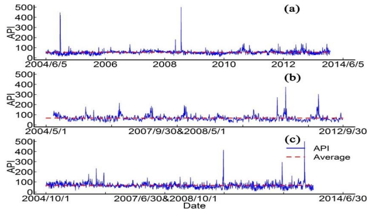
Figure 6: The typical characteristics of Saltatory-quality. (a) Kelamayi, (b) Yangzhou, (c) Deyang.
