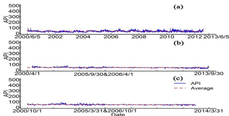
Figure 8: The typical characteristics of ideal-quality type. (a) Haikou, (b) Beihai, (c) Zhanjiang.
