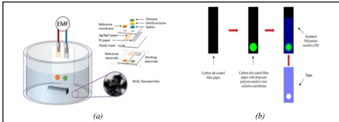
Figure 3: (a) Paper-based electrodes for the detection of galactose in blood [11] (b) Paper-based electrodes for poly anion detection [12]
