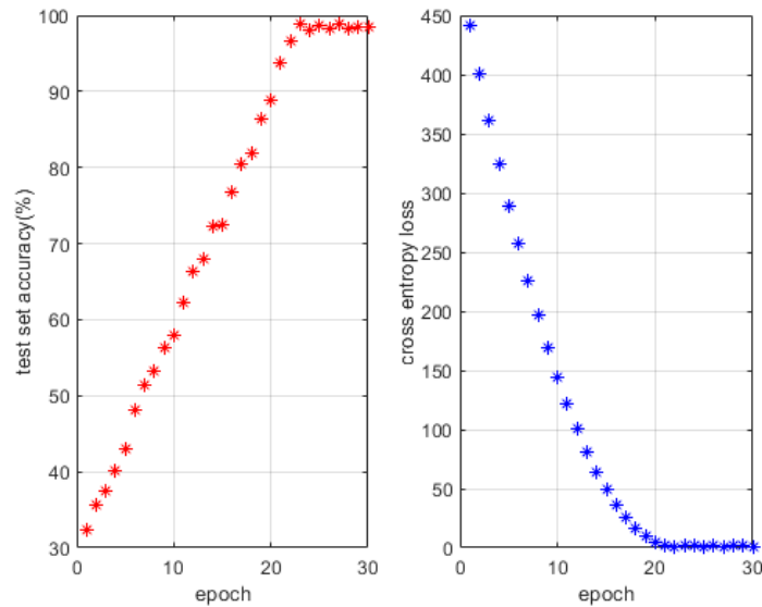
Figure 3: Variation trend of loss value and test set accuracy with training algebra
