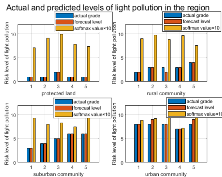
Figure 4: Bar chart comparing the predicted light pollution level with the actual level
