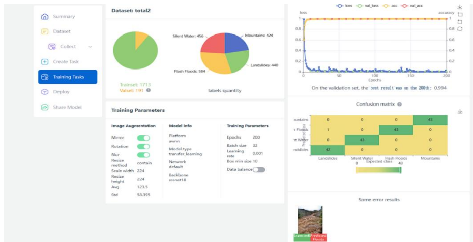
Figure 3: Model Training
