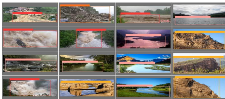
Figure 4: Image recognition
