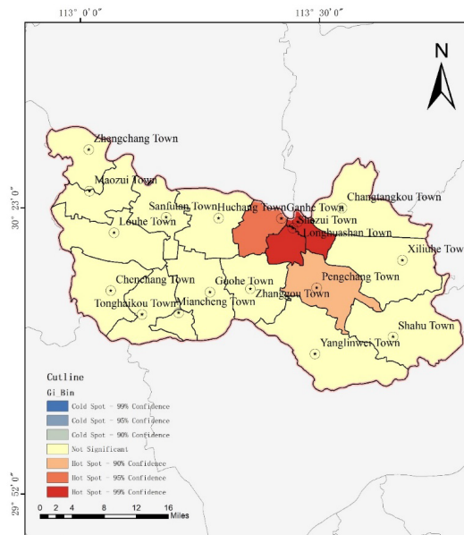
Figure 6: Hotspot and Coldspot Cluster Map
