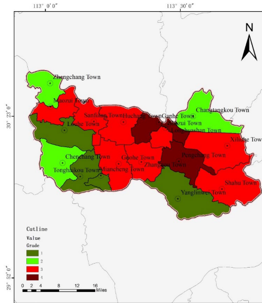
Figure 5: LISA Cluster Map
