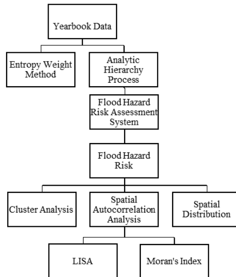
Figure 1: Is based on the spatial pattern analysis model using SPSS and ArcGIS.
