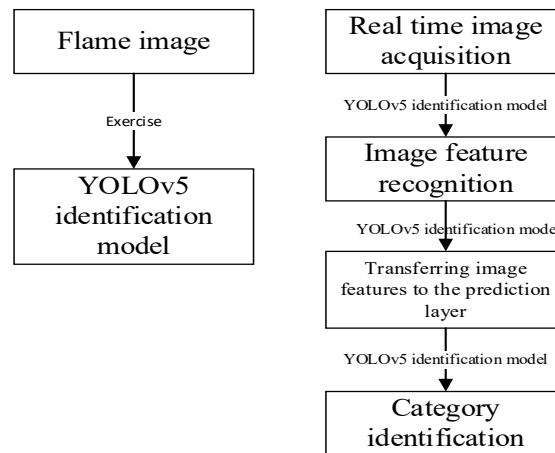
Figure 12: Flame recognition process
