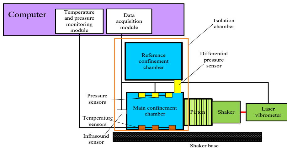
Figure 1: Scheme of laser absolute method infrasound calibration device.
