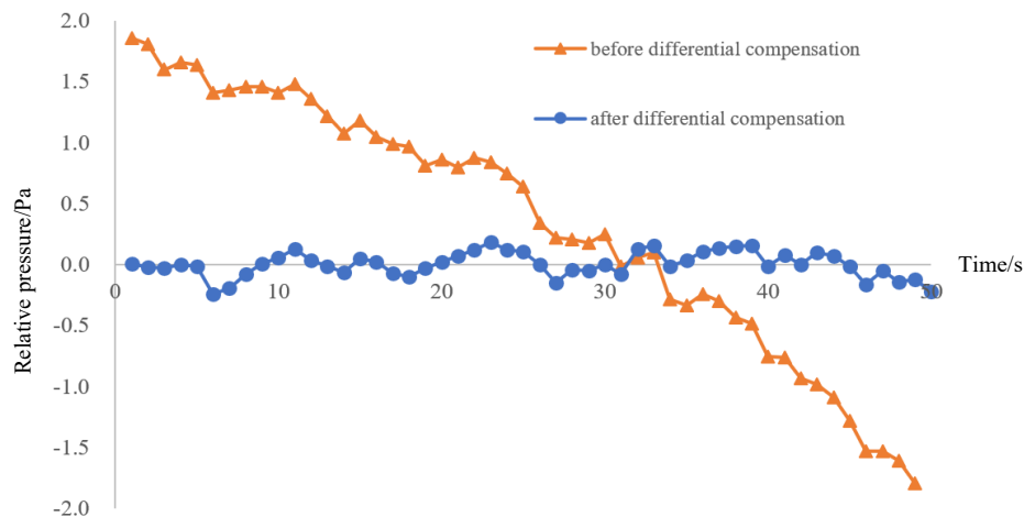
Figure 4: Main confinement chamber pressure waveform before and after differential compensation.
