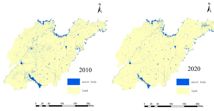
Figure 6: Results of water extraction in Shandong Province in 2010&2020
