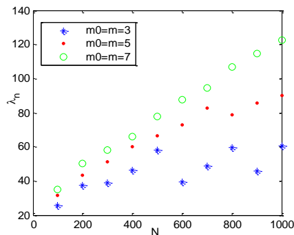
Figure. 2 The relationship between network size N and the minimum value of \lambda_n .
