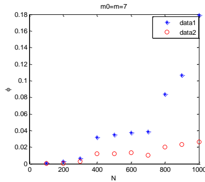
Figure.3 Relationship between network scale and consistency convergence time of BA scale-free network model and BA-based synchronous optimal network model
