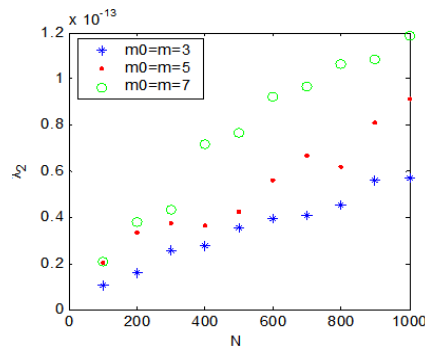
Figure.1 Relationship between the network size N and the maximum value of \lambda_2
