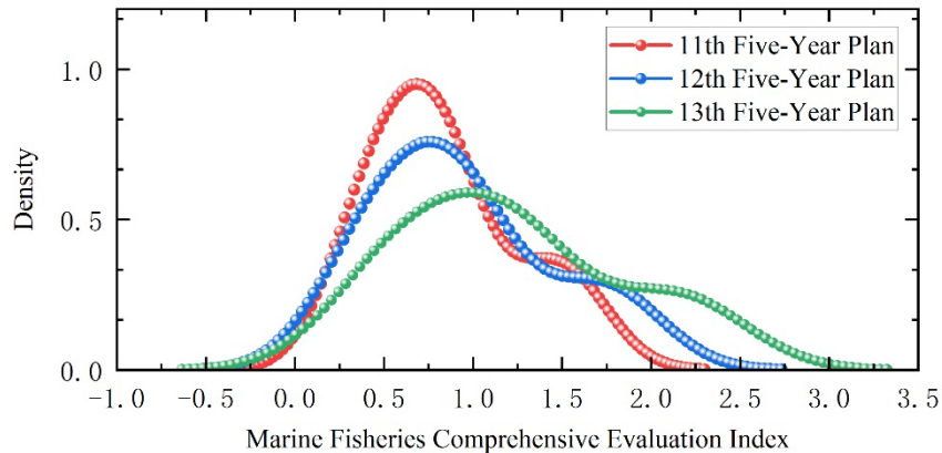
Figure 2: Kernel Density Curve of China's Marine Fisheries Comprehensive Evaluation Index
