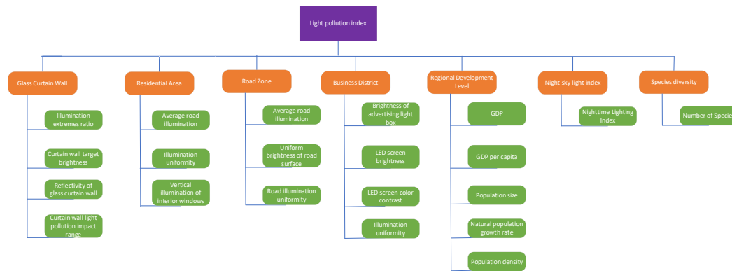
Figure 1: Structure of light pollution evaluation index system
