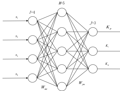
Figure 3: Structure diagram of BP neural network
