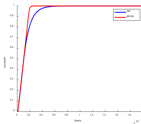
Figure 5: Ideal environment
