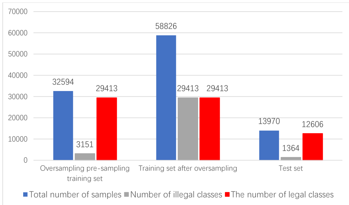
Figure 3: Une balanced dataset processing results
